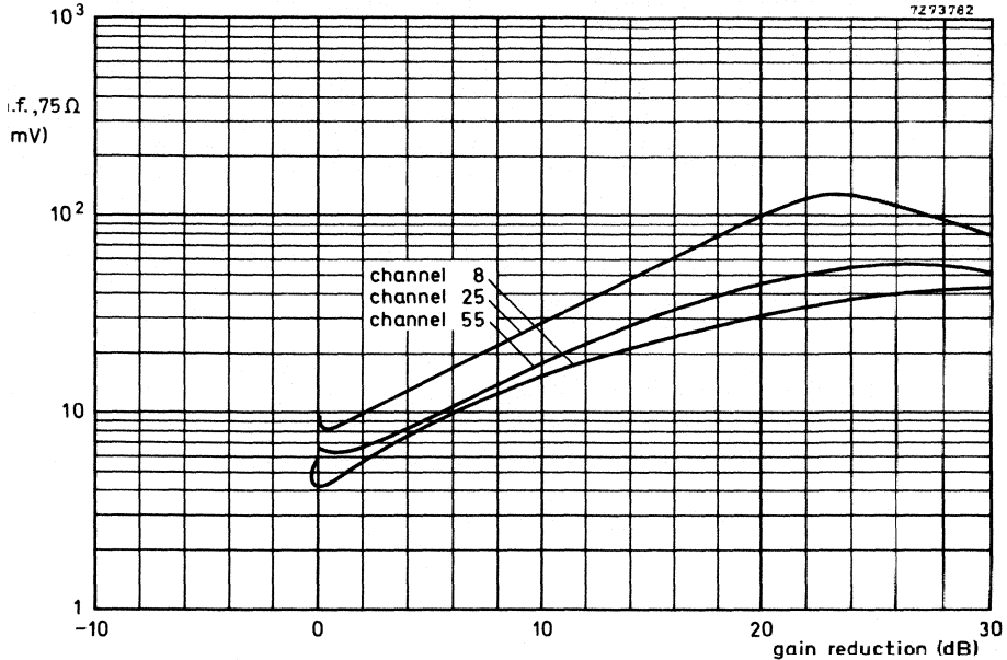
Fig. 10. Cross-modulation, in channel.
