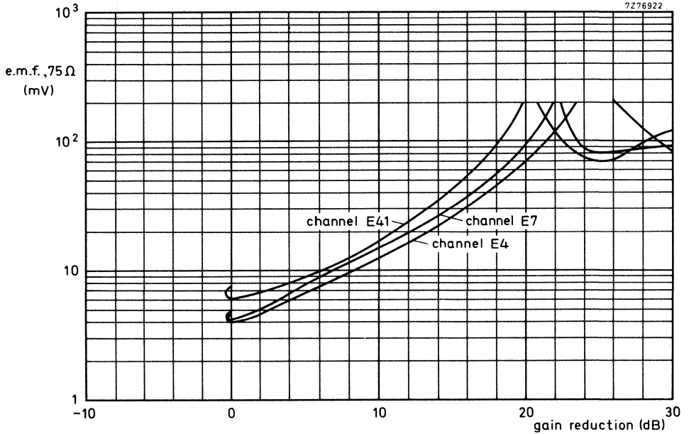
Fig. 12 Cross-modulation, in channel.
