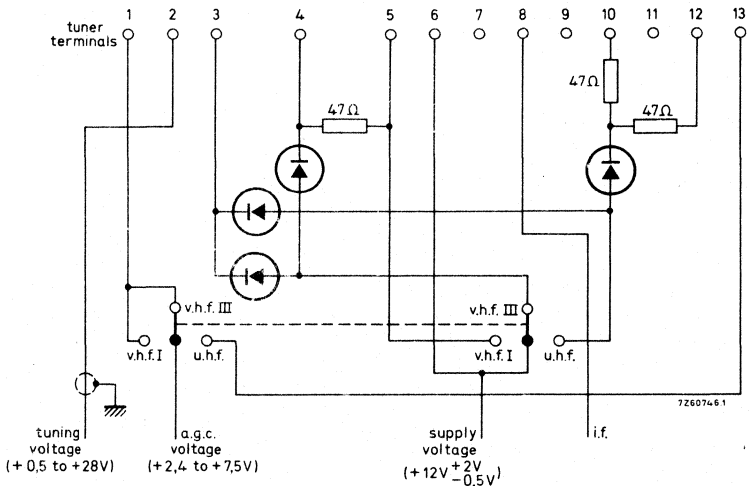
Fig. 15. Connection diagram with two switches. All diodes: BAX13, BA217 or comparable silicon diodes.
