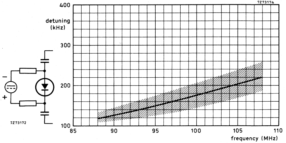
Fig. 8 Detuning as a function of signal frequency at a control voltage change from 0 to -400 mV.
